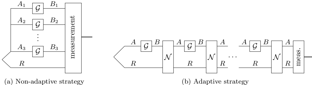
Figure 2: Two general protocols for non-adaptive and adaptive strategies for the task of channel discrimination. The channel \mathcal{G} is either \mathcal{E} or \mathcal{F} and the task is to distinguish between these two cases.
