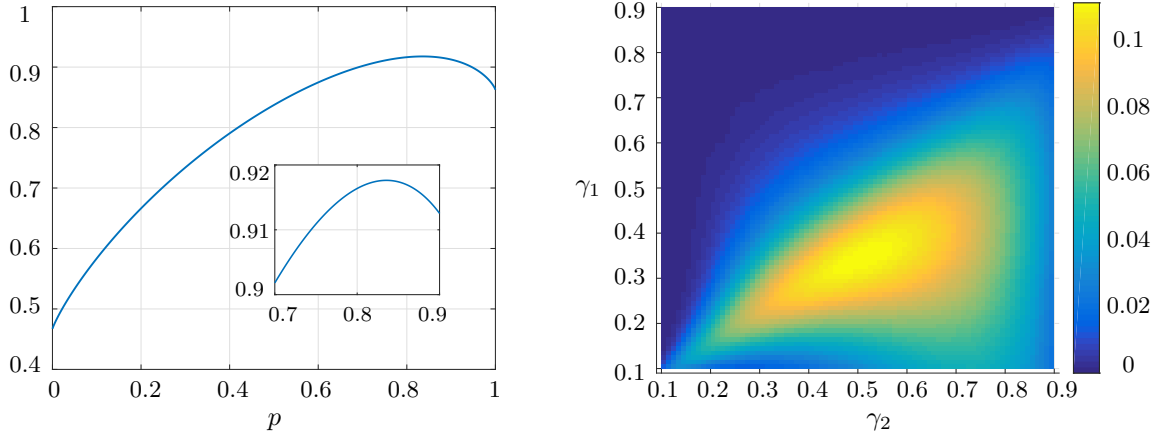
Figure 1: The left figure plots of the value D(\sqrt{\rho_R} J_{RB}^{\mathcal{E}} \sqrt{\rho_R} \| \sqrt{\rho_R} J_{RB}^{\mathcal{F}} \sqrt{\rho_R}) with respect to the input state \rho_R = \text{diag}(p, 1-p) . The subfigure is a zoom in plot with the parameter ranging from 0.7 to 0.9. It is evident that D(\mathcal{E}\|\mathcal{F}) cannot be larger than 0.92. The right figure shows a heat map of the value D(\mathcal{A}_{\gamma_1,0}^{\otimes 2} \| \mathcal{A}_{\gamma_2,0.9}^{\otimes 2}) - 2D(\mathcal{A}_{\gamma_1,0} \| \mathcal{A}_{\gamma_2,0.9}) where \gamma_1, \gamma_2 \in [0.1, 0.9] . This shows that the non-additivity behavior of the channel relative entropy under tensor products occurs for many channels.
